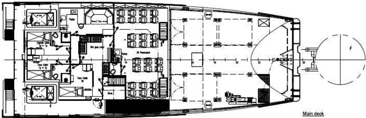
Main deck
